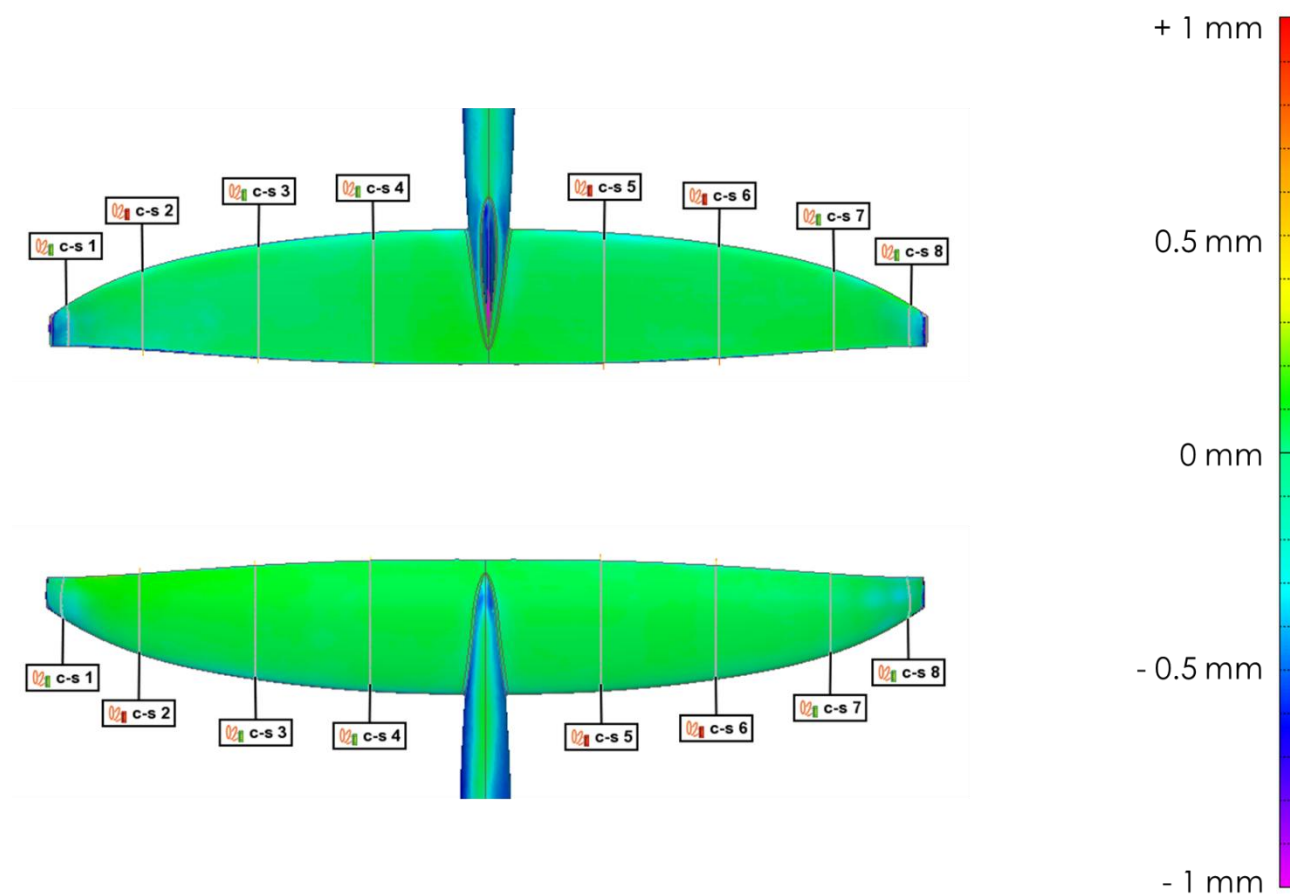
Figure 6 - Colour Map of the Upper (top) and Lower (bottom) surfaces of the Rearwing
