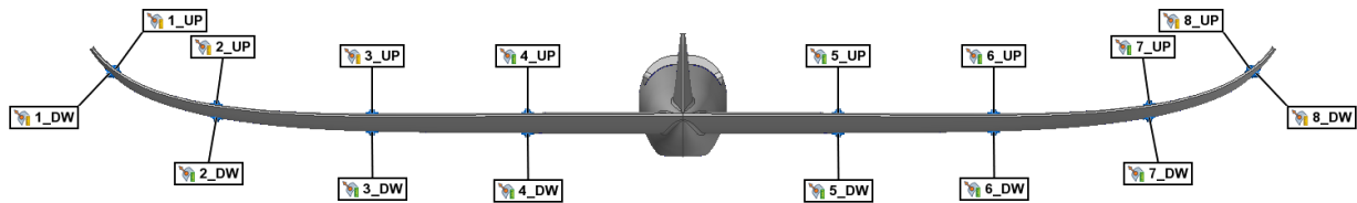
Figure 4 - Surface Distance Points definition
