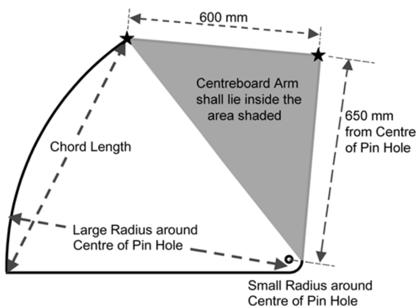
E.2.5 (a). CENTREBOARD DIMENSIONS
