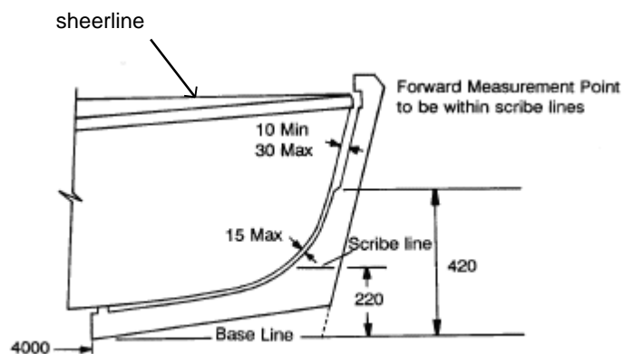
Stem Measurement
