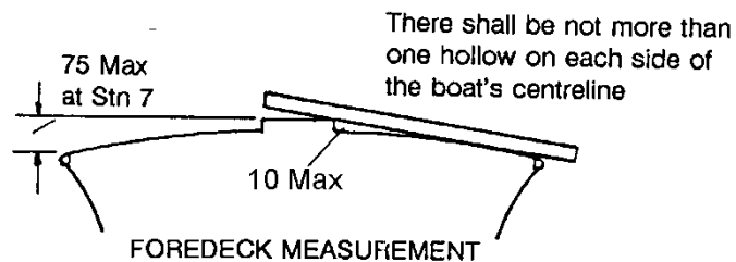
Foredeck Measurement
